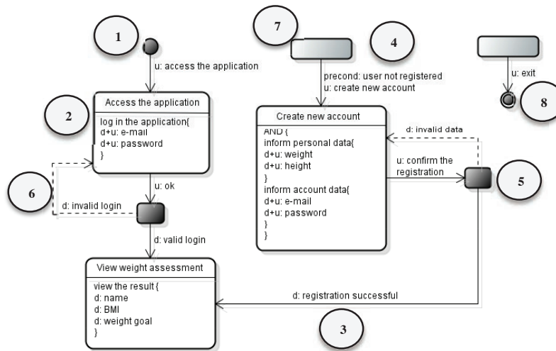
Figure 1. A MoLIC diagrams example.
